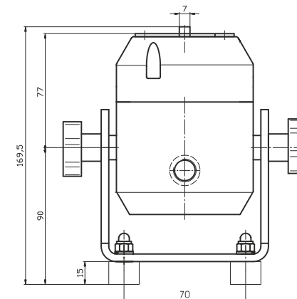
S 50018 (Example drawing) (mm)
